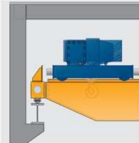
Standard main girder connection configuration - Version 1
