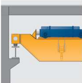
Stooled down configuration*
